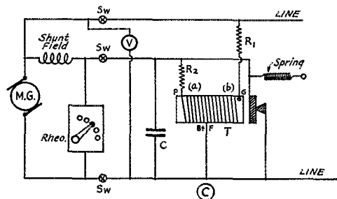
FIG. 4 — VOLTAGE REGULATOR FOR THE MOTOR-GENERATOR SET MADE FROM AN AUDIO TRANSFORMER AND FORD CONTACTS T — 6-1 audio transformer (Thordarson). Secondary winding at (b); primary winding at (a).
