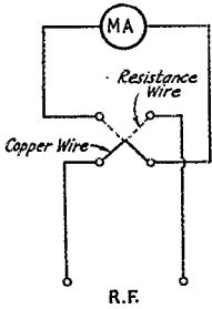
FIG. 4—R. F. MEASUREMENTS USING THE THERMOCOUPLE AND D.C. MILLIAMMETER
